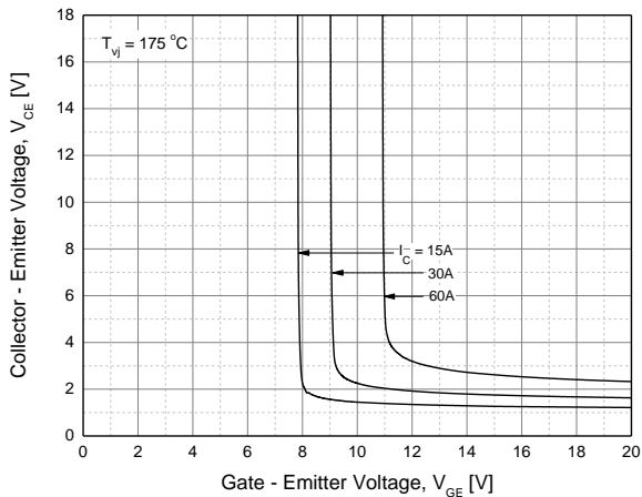
Fig. 5 IGBT Saturation Voltage vs. Gate Bias
